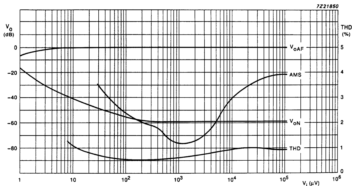
Fig.18 Signal and noise ( V_{OAF} ), noise ( V_{ON} ); reference level 0 dB = 100 mV; AM suppression (AMS) and total harmonic distortion (THD) as a function of input voltage ( V ) at pin 1. Measured in test circuit Fig.5 at f_i = 98 \text{ MHz} ; f_{\text{mod}} = 1 \text{ kHz} ; \Delta f = 22.5 \text{ kHz} . AM suppression is measured at f_{\text{mod}} = 400 \text{ Hz} , m = 0.3 for AM; f_{\text{mod}} = 1 \text{ kHz} , \Delta f = 75 \text{ kHz} for FM.
