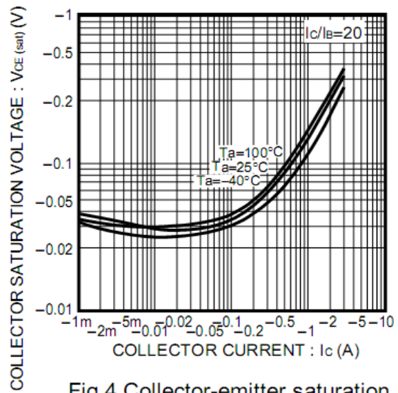
Fig.4 Collector-emitter saturation voltage vs. collector current
