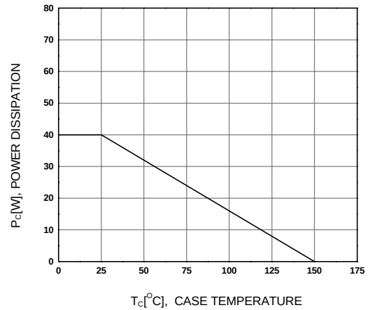
Figure 6. Power Derating
