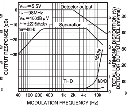
Fig. 24 Fidelity characteristics
