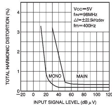
Fig. 27 Sensitivity characteristics
