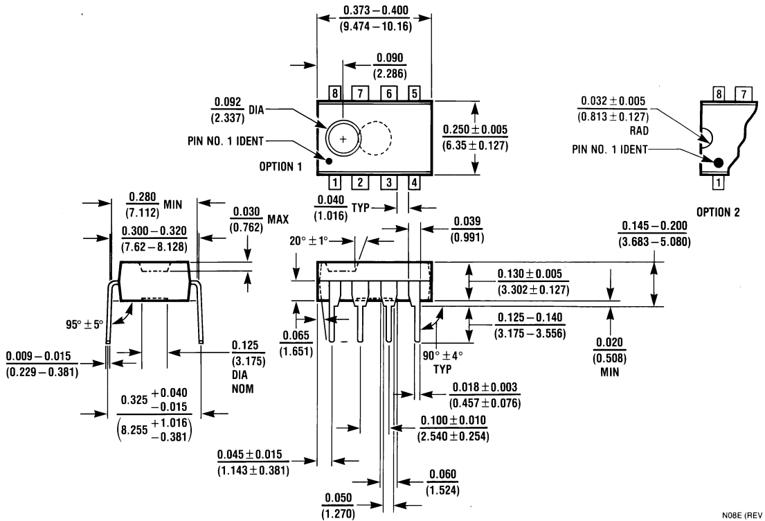
Molded Dual-In-Line Package Order Number LF353N NS Package Number N08E
