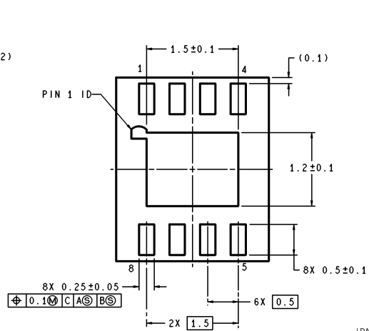
8-Pin LLP NS Package Number LDA08C
