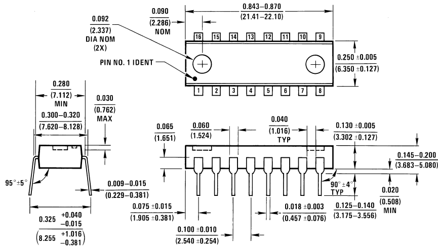
16-Pin Plastic Dual-In-Line Package Order Number LP2956IN or LP2956AIN NS Package Number N16A
