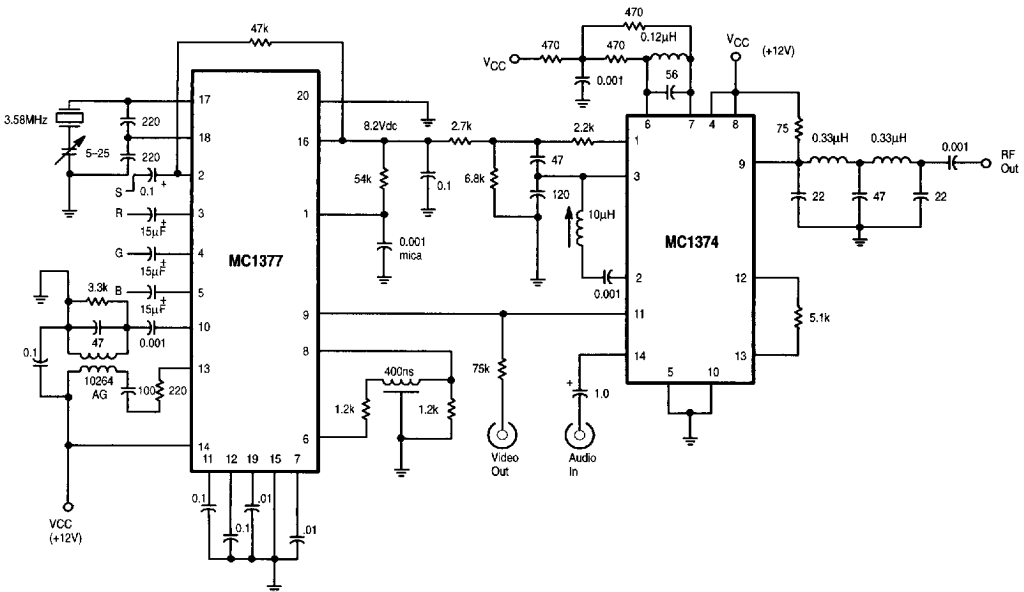
Figure 27. Color TV Encoder - Modulator
