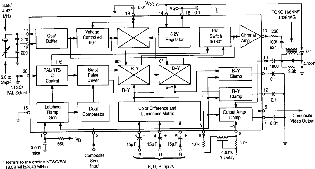
Figure 7. Block Diagram and Application Circuit
