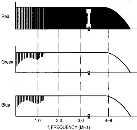
Figure 17. Spectra of a Full RGB System
