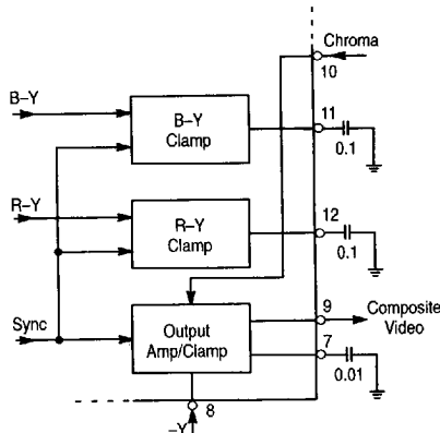
Figure 7. Block Diagram and Application Circuit
