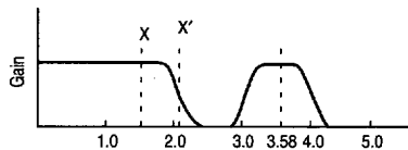
(b) Standard Receiver Response
