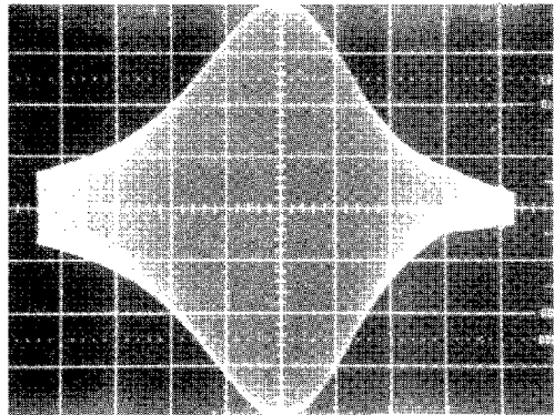
Figure 19. Frequency Response of Chroma Coupling Circuit
