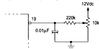
Figure 10. Adjusting Modulator Angle
