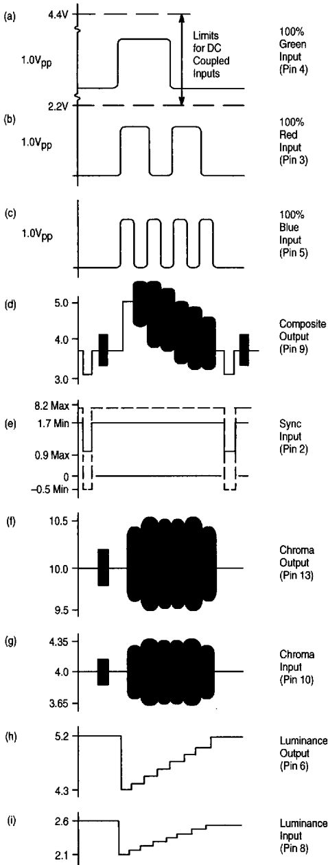
Figure 8. Signal Voltages (Circuit Values of Figure 7)
