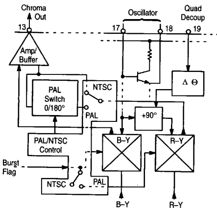
Figure 4. Chroma Section
