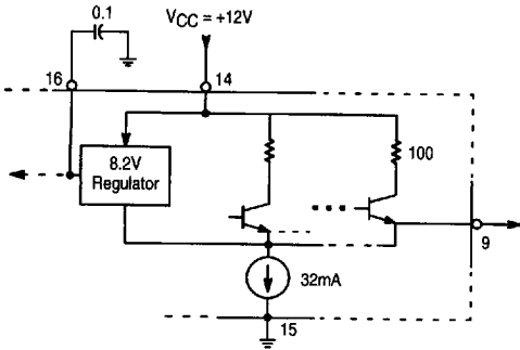
Figure 2. Power Supply and V_B
