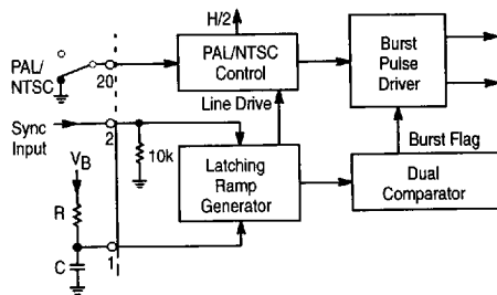
Figure 5. Timing Circuitry
