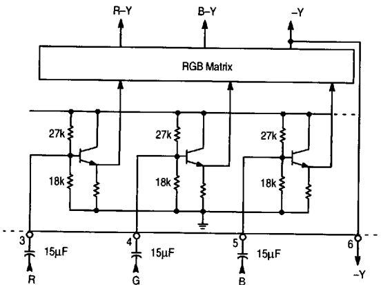
Figure 4. Chroma Section
