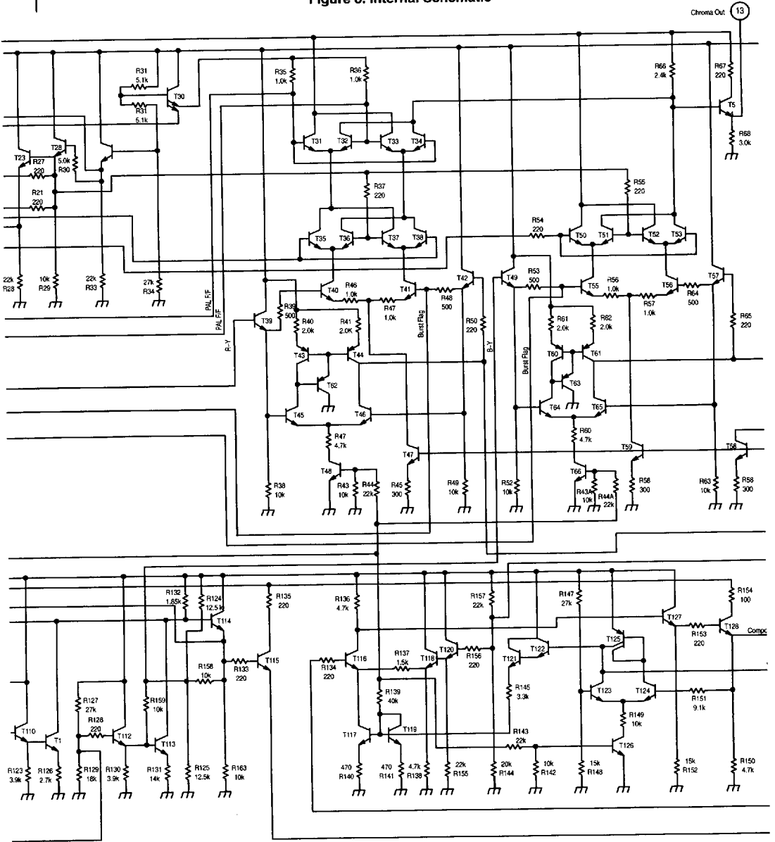
Figure 8. Internal Schematic
