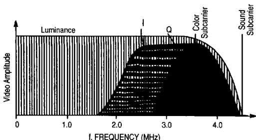
Figure 20. NTSC Standard Spectral Content
