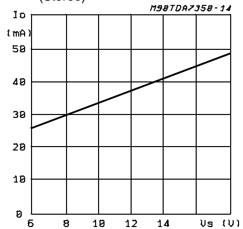
Figure 10: Drain Current vs Supply Voltage (Stereo)
