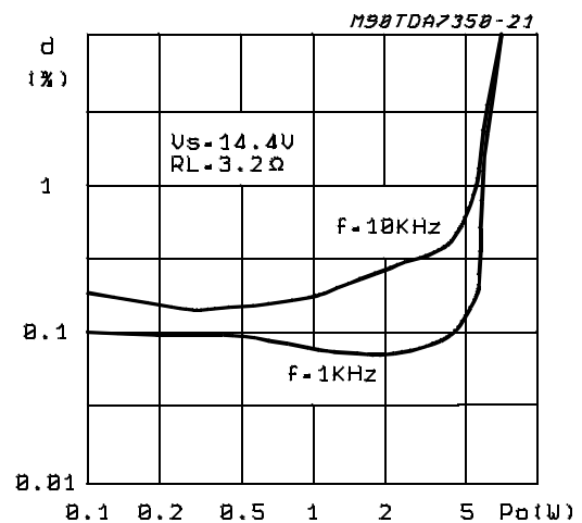
Figure 12: Distortion vs Output Power (Stereo)
